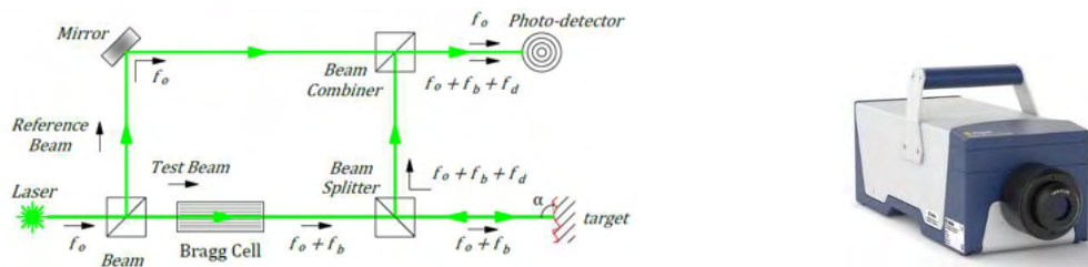
Figure 14: (a) Laser Doppler Vibrometer operation schematic, (b) Polytec single point vibrometer head
