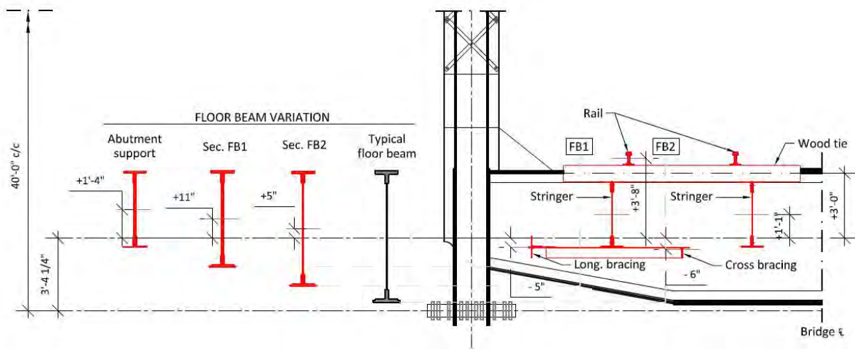
Figure 33: Devon bridge: Floor system and cross-section variation
