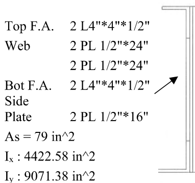
(f). Typical section; Node L2-L3, L5-L6 (Bottom Chord)
