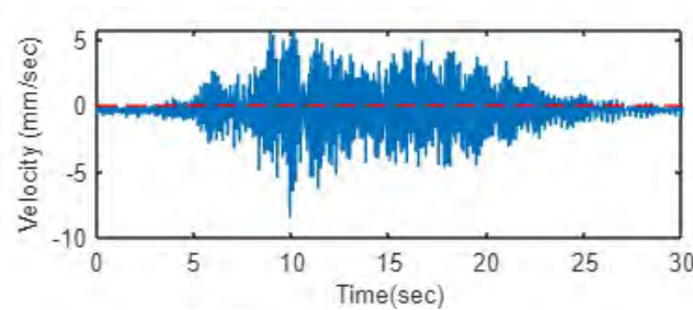
Figure 26: Lateral velocity-time response at Vib. Loc 4 under/subjected to 10-car Metro North train moving at 21 mph from New York to New Haven on track 4 of Cos Cob bridge, CT
