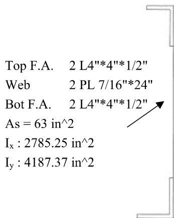
(d). Typical section; Node L0-L1, L7-L8 (Bottom Chord)
