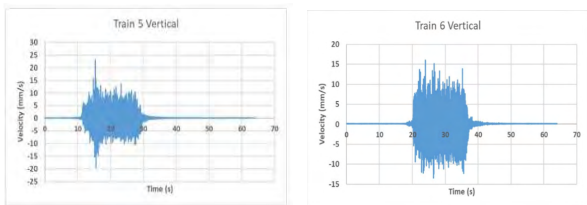
Figure B- 1: Velocity-time response at node Vib.1 under/subjected to 8-car Metro North train moving at 37.87 mph from New York to New Haven on track 4 of Cos Cob bridge, CT (left) and at node Vib.2 under/subjected to 8-car Metro North train moving at 42.41 mph from New York to New Haven on track 4 of Cos Cob bridge, CT.
