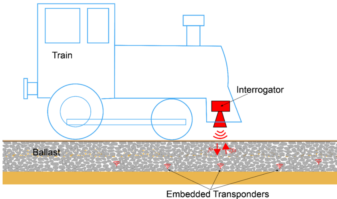
Figure 13: Conceptual field deployment of the passive wireless tag for railbed monitoring
