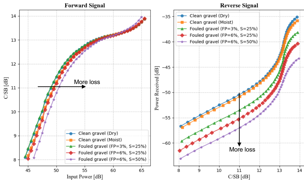
Figure 7: CSB vs input power from forward signal at 1.2 GHz (left) and power received vs CSB from reverse signal at 2.4 GHz (right) for clean and fouled gravels
