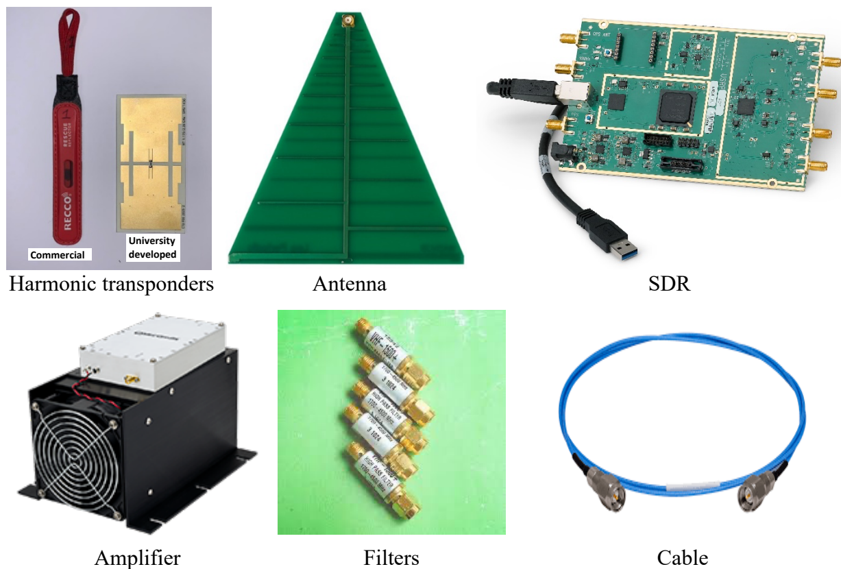
Figure 4: Components of the electrical measurement system
