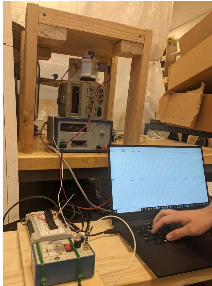
Figure 1. Acoustic sensor arm undergoing testing of upgrades on concrete slab in laboratory
