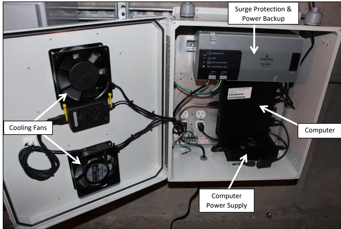
Figure 4. Inside of the computer junction box located at the Pylon base station.
