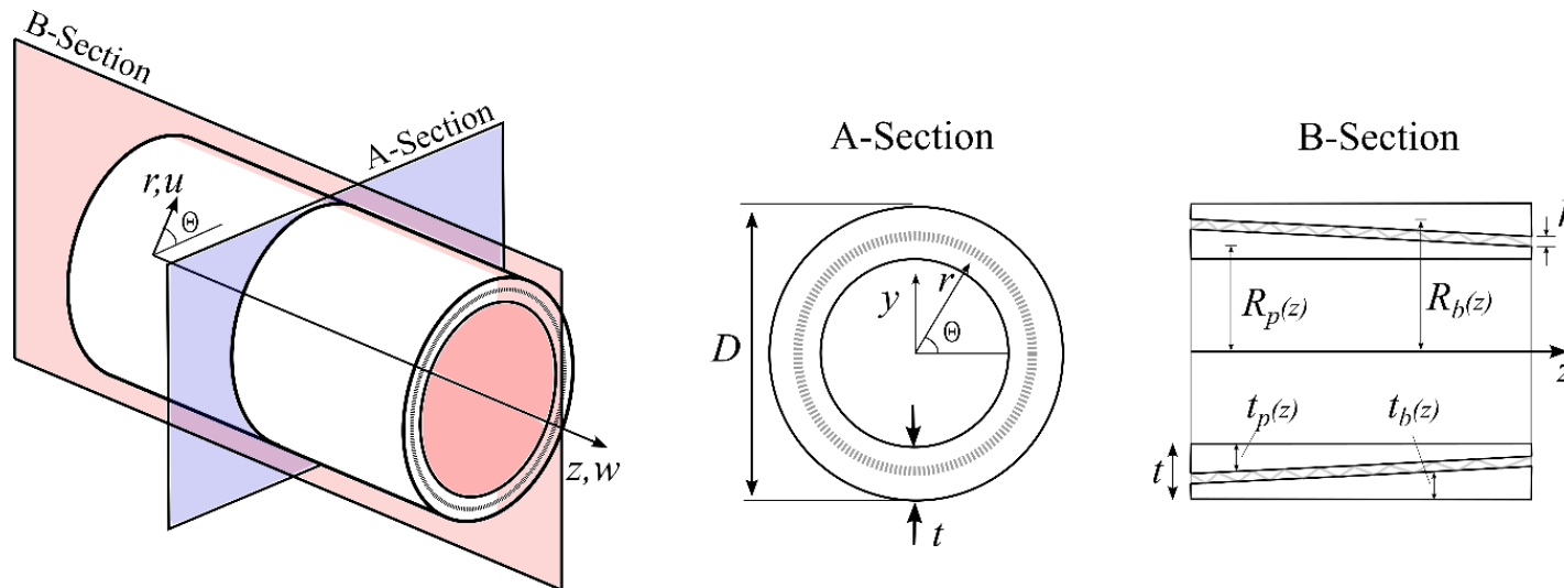
Figure 1 Simplified analytical model of threaded joint.
