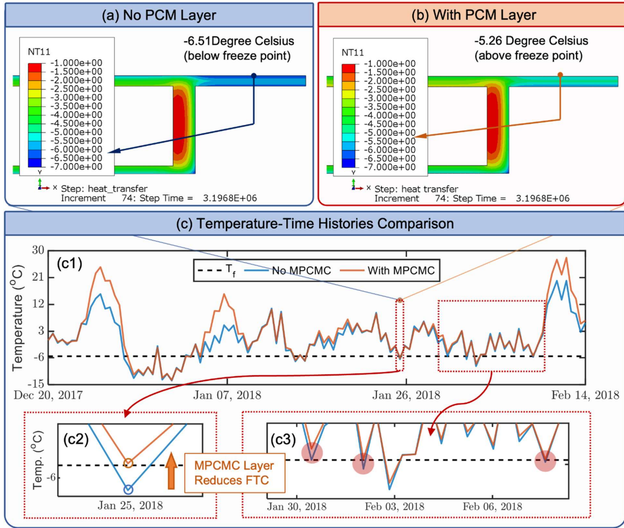
Fig. 21 The effectiveness of the proposed MPCMC protective layer by comparing the control case with respect to an exemplary layer with design parameters: d_{\text{pcm}} = 8 \times 10^{-6} \text{ m} , v_{\text{pcm}} = 0.05 , \rho_{\text{eff}} = 2213 \text{ kg/m}^3 , k_{\text{eff}} = 1.21 \text{ W/m} \cdot \text{K} , C_{\text{peff}} = 908.9 \text{ J/kg} \cdot \text{K} , t_{\text{ol}} = 0.036 \text{ m} , H = 250 \text{ kJ/kg} \cdot \text{K} , and T_t = -5 . (a) The temperature field without the MPCMC; (b) the temperature field with the exemplary MPCMC; (c) a comparison of the temperature-time histories with and without the MPCMC layer with close-ups that illustrate the FTC reduction about the freezing temperature T_f . Figure c1 shows the overall temperature-time histories. Figures c2 and c3 show close-ups of the Figure c1 at two different time ranges.
